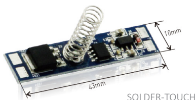
SOLDER-TOUCH
